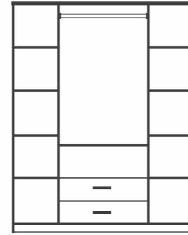
4 kapaklı gardrop / 4-door wardrobe E/W 1600 B/H 2000 D/D 600
