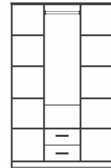
3 kaplı gardrop / 3-door wardrobe E/W 1250 B/H 2000 D/D 600
